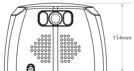
INSTALLATION TEMPLATE
