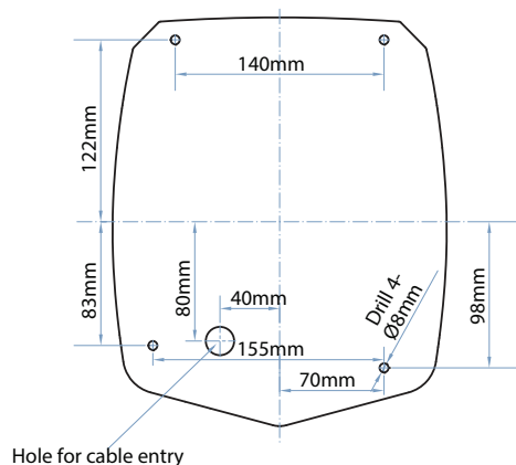
INSTALLATION TEMPLATE
