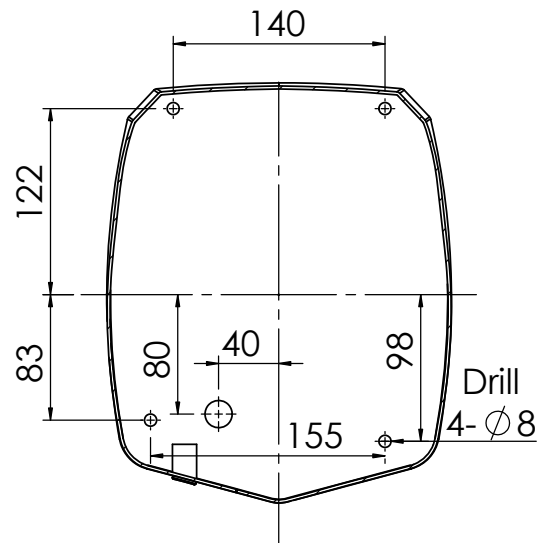
INSTALLATION TEMPLATE
