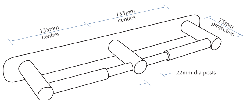
Model R023-BP-MB with backplate
