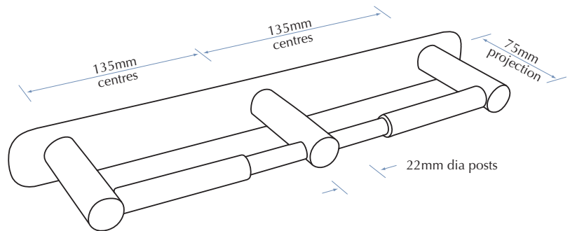
Model R023-BP with optional back plate
