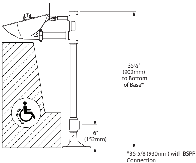
Eyewash Bowl
